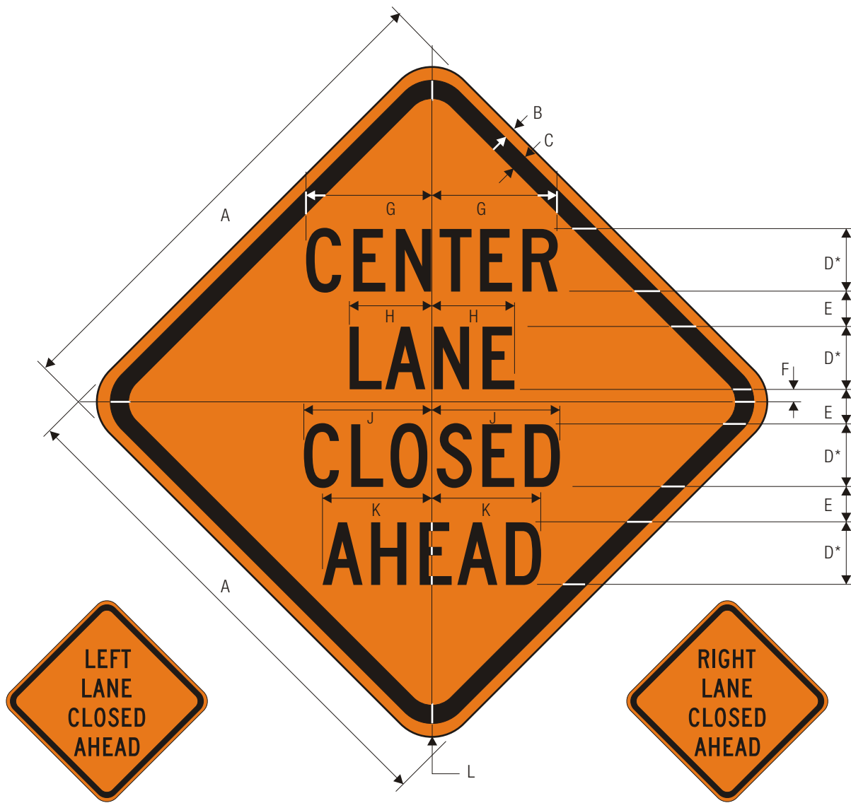
W9-3L
