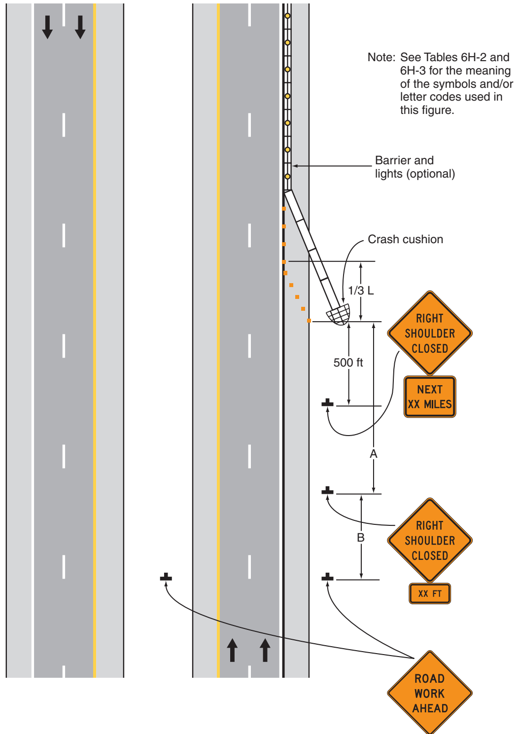
Figure 6H-5. Shoulder Closure on a Freeway (TA-5)
