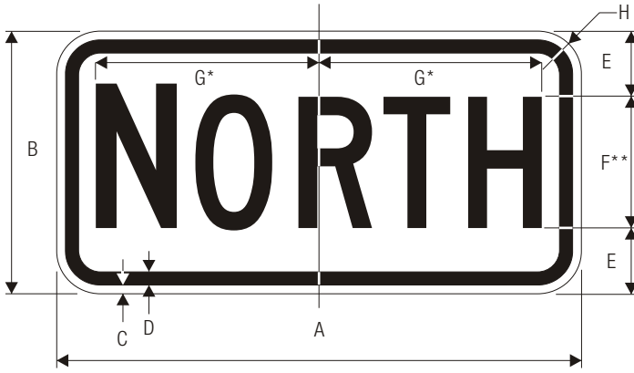
M3-1 CARDINAL DIRECTION AUXILIARY
