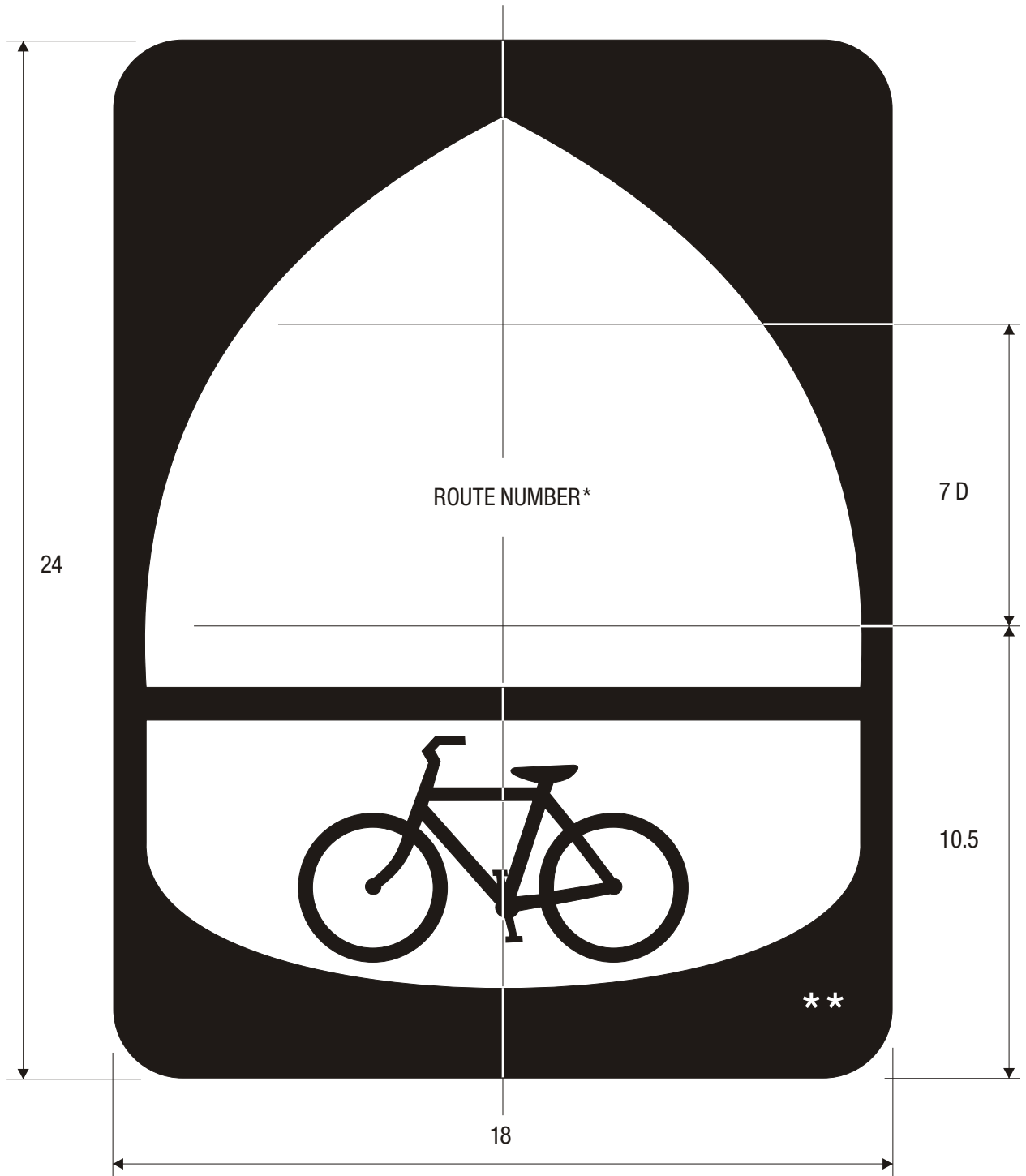
M1-9 BICYCLE ROUTE
