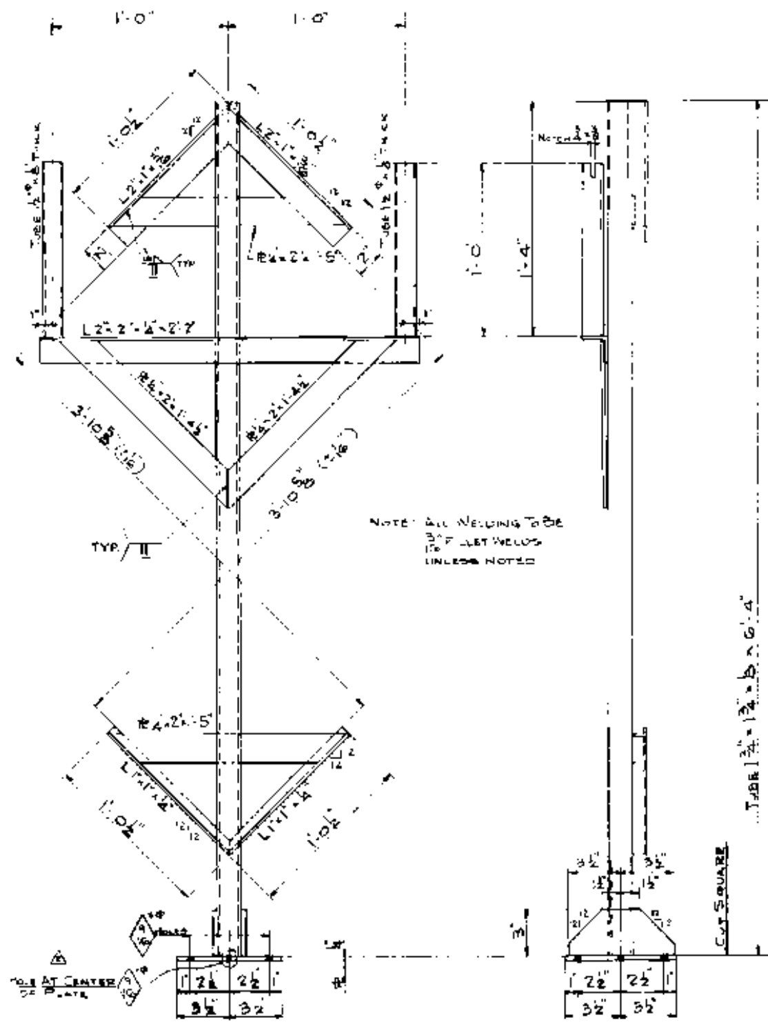
FRONT VIEW
